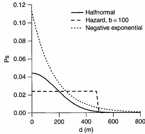
Fig. 2 Detection functions p_s(d) fitted to stoat data from proximity detectors in the Matakaitaki Valley, New Zealand, where d is the distance between an animal's home range centre and a detector. Density estimates (Table 3) were stable despite the considerable variation in the fitted detection functions
